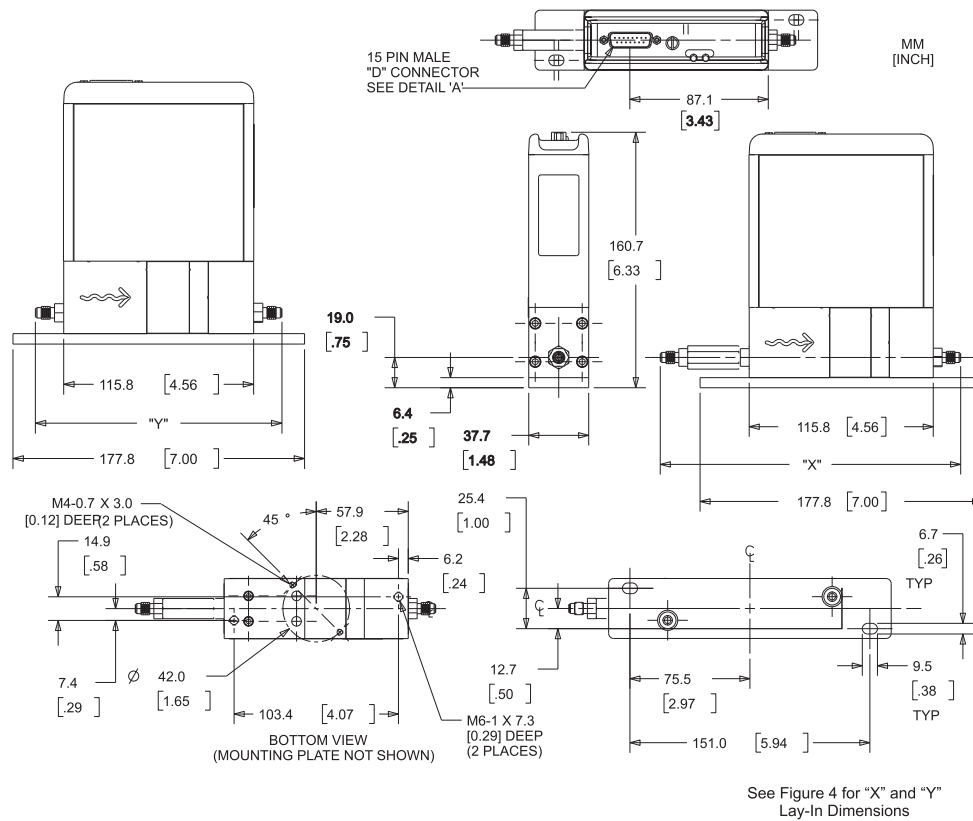
Figure 2 Dimensional Drawing QmB IP40
