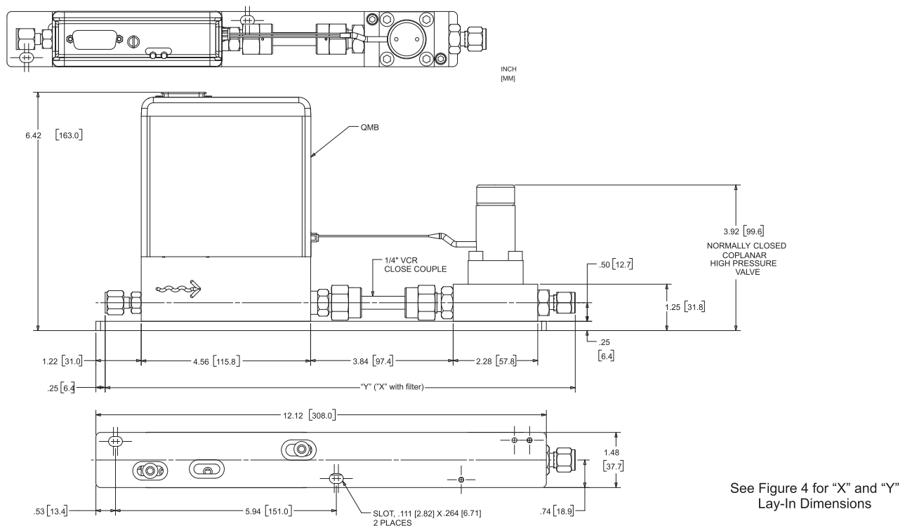
Figure 5 Dimensional Drawing QmB IP40 with Remote Valve
