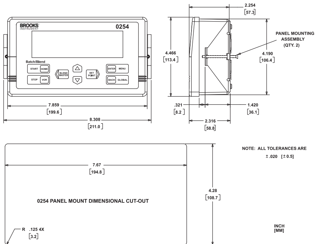
Model 0254 Panel Mount Dimensions
