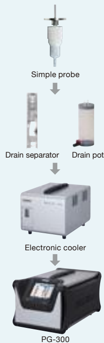
Stack gas
